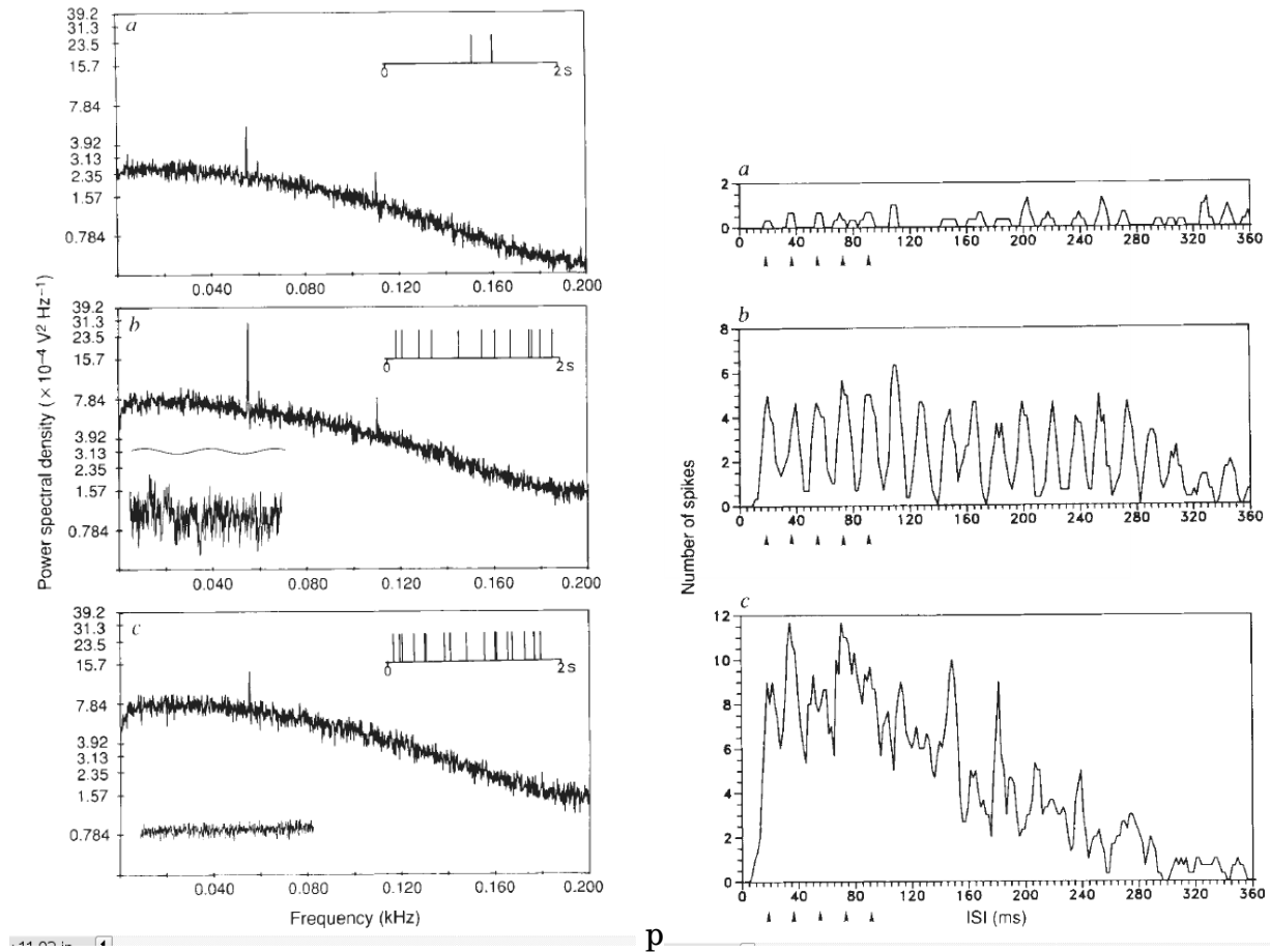
Figure 5: a) Power spectrum from spiking activity of crayfish mechanoreceptor for 3 different noise levels with fixed weak periodic signal. b) Interspike interval histograms for different noise levels [12].
