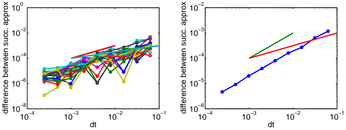
Figure 10: Milstein scheme for dy = -0.2y dt + y dW : a) errors for 20 individual realizations of the Wiener process as a function of \Delta t . b) mean error.
